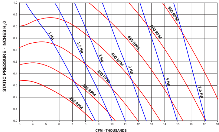
ID/IS601 w/ WS080 - Airflow Data
